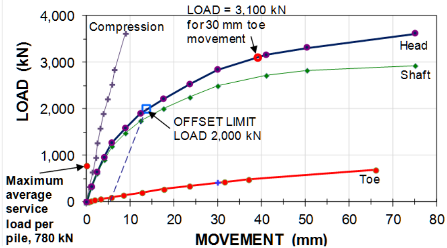
Fig. 9 Results of the static loading test: Load-movements of pile head, pile toe and shaft, Case 2
