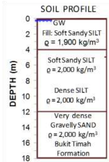
Fig. 14 Soil profile at the Singapore site, Case 3
