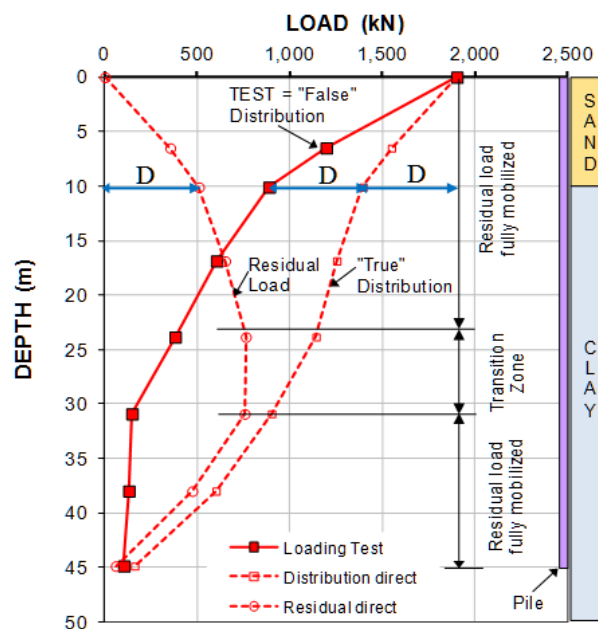
Fig. 6 "False", "True", and Residual force Distributions, Case 1. The double-arrows labeled "D" indicate values of equal load.
