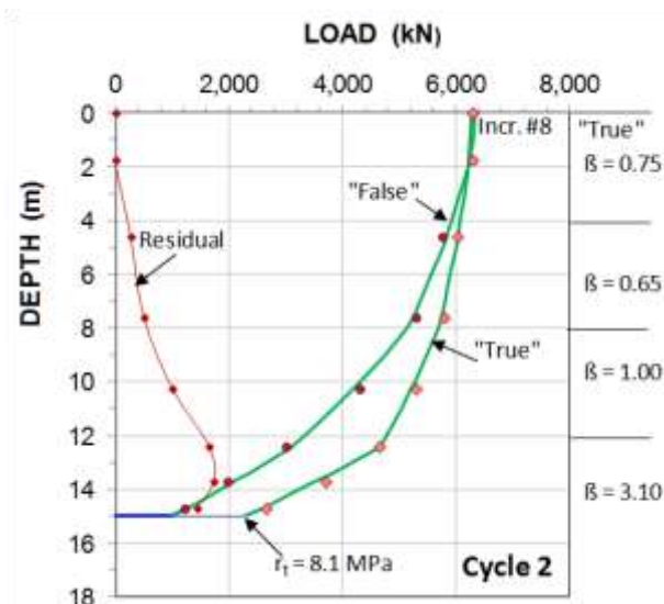
Fig. 17 "False", "True", and Residual force distributions; Cycle 2 with back-calculated beta-coefficients, Case 3
